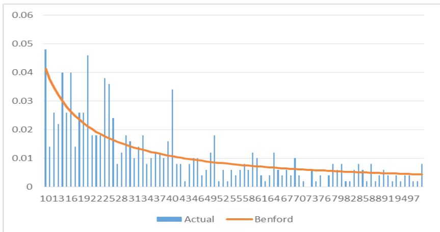
Figure 3: Proportion of F2D Test of 500 Payment Vouchers
